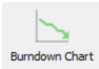
Burndown Chart
